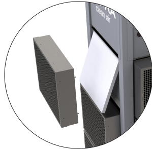
ASPRA L-C Mobile - cartridge detail
